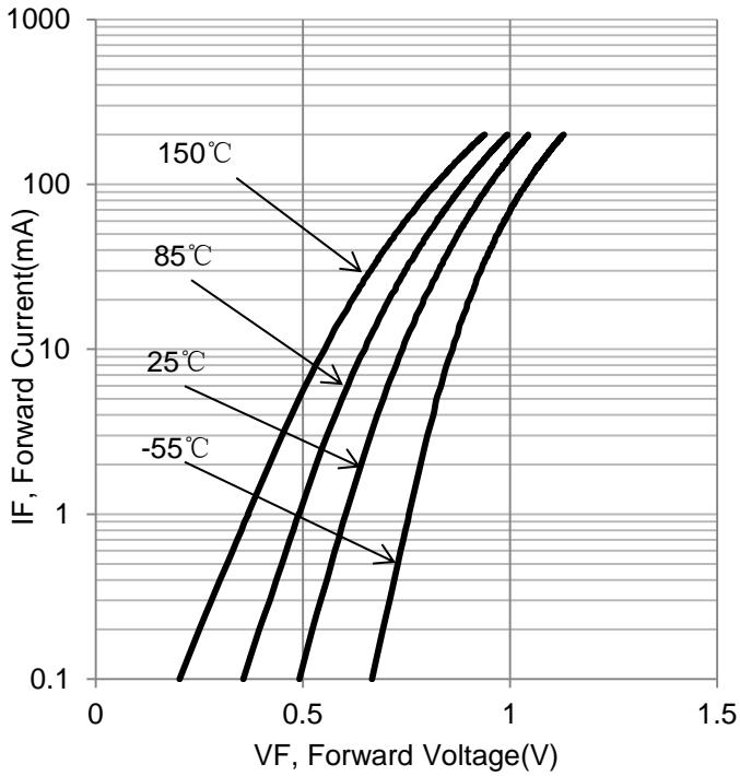
Forward Characteristics
