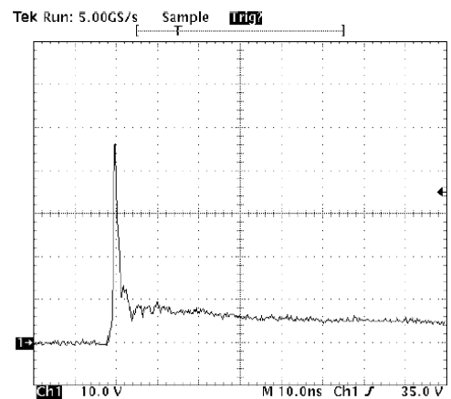
Note: Data is taken with a 10x attenuator ESD Clamping Voltage
