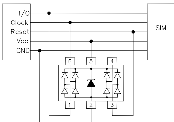
Figure 6 - SIM Port
